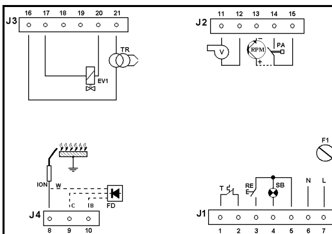
Type TGRD81
