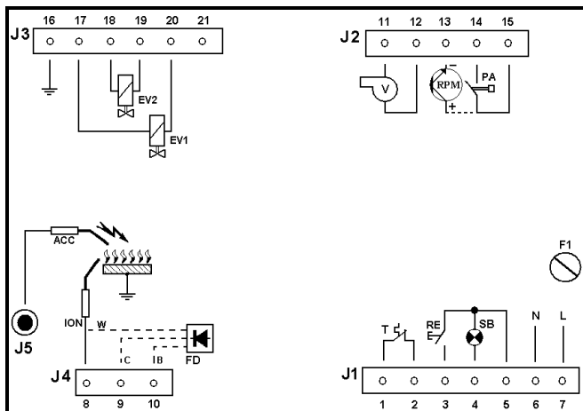
Type TGRD62
