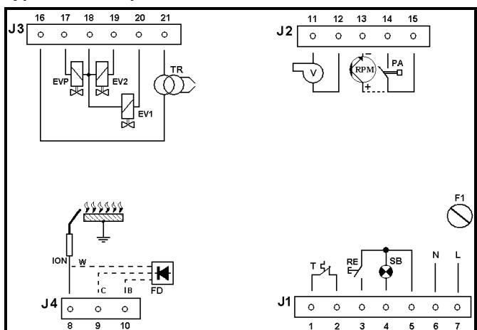
Type TGRD83
