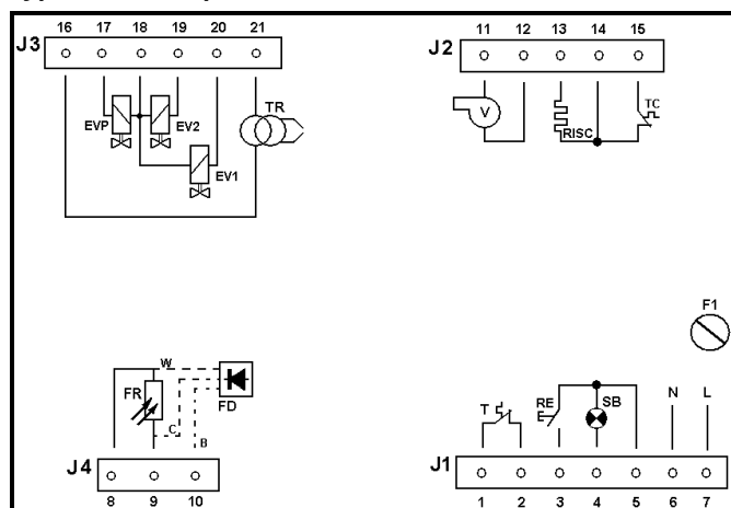
Type TGRD93
