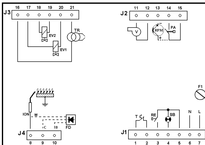
Type TGRD82
