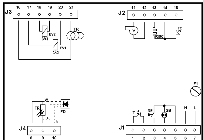
Type TGRD92
