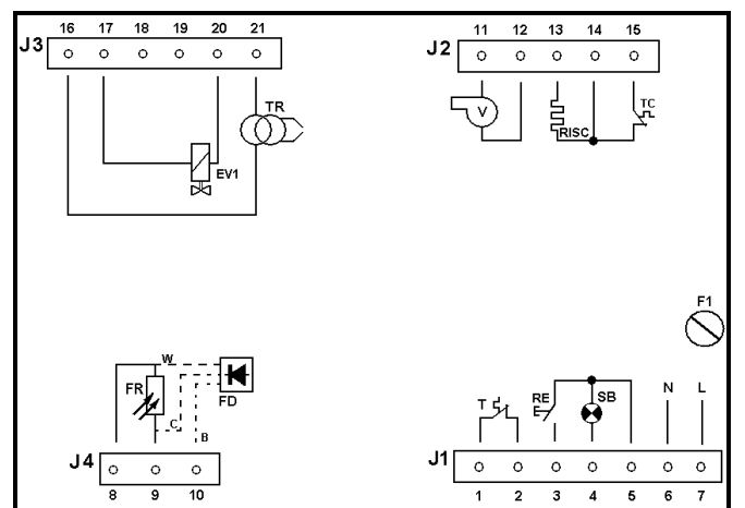
Type TGRD91
