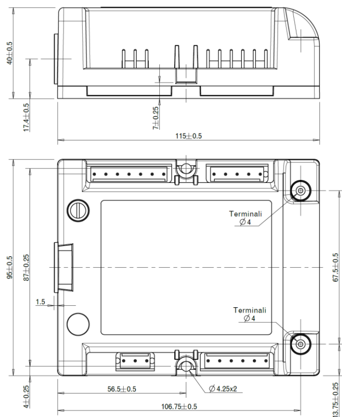
Fig. 1 – Overall dimensions
