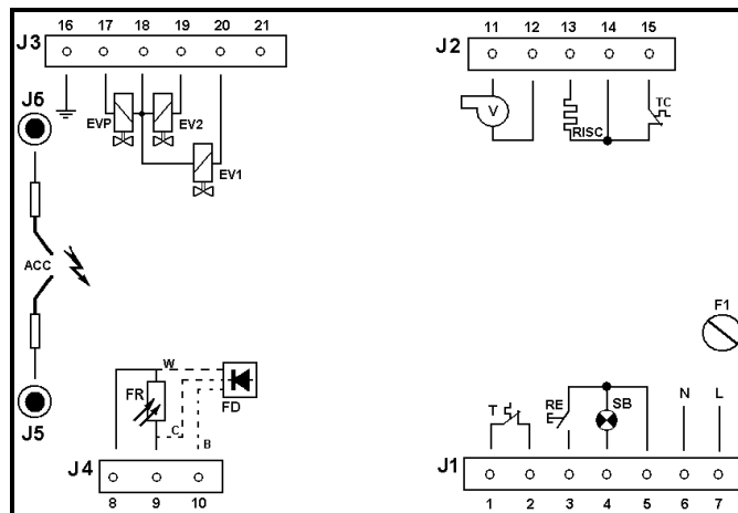
Type TGRD73
