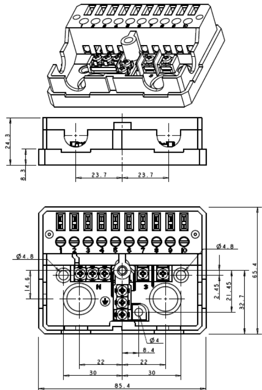
N Socket Fig.2
